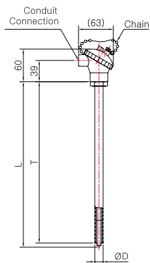
Model No. | SS-5014S-2-1 ( Metal Protection Tube )
