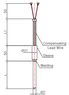
Model No. | SS-5048GD ( Sheath )
