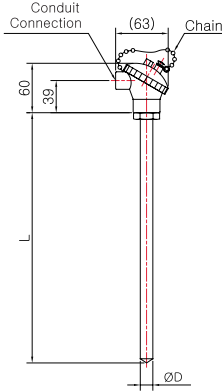
Model No. | SS-5041S (Sheath)
