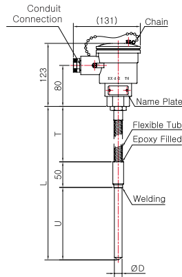
Model No. | SS-5029E (Sheath)
