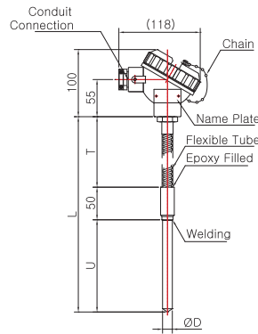
Model No. | SS-5049W (Sheath)
