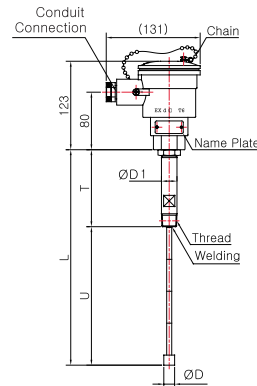
Model No. | SS-5015E ( Metal Protection Tube )
