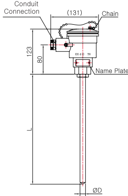
Model No. | SS-5041E (Sheath)
