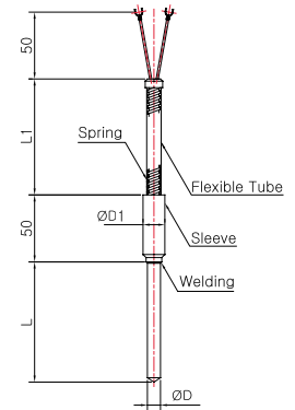
Model No. | SS-5048GE ( Flexible Tube )
