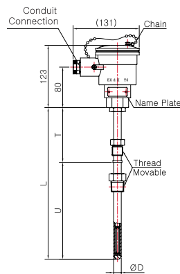
Model No. | SS-5032E-3 ( Metal Protection Tube )
