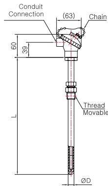
Model No. | SS-5016S-2 ( Metal Protection Tube )
