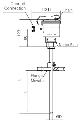
Model No. | SS-5049E (Sheath)
