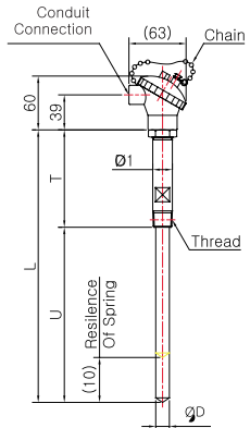
Model No. | SS-5044S-1 (Sheath)
