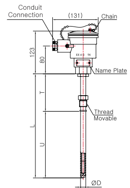
Model No. | SS-5012E-2 (Metal Protection Tube)
