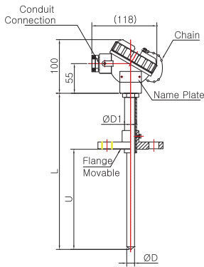
Model No. | SS-5046W-2 (Sheath)
