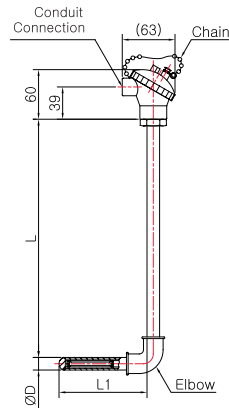
Model No. | SS-5037S ( Metal Protection Tube )
