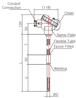
Model No. | SS-5019W ( Metal Protection Tube )
