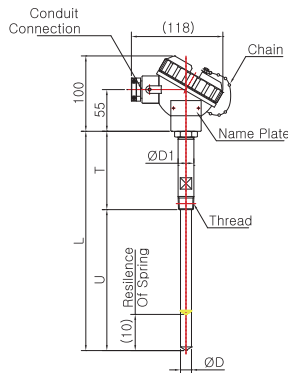
Model No. | SS-5044W-1-1 (Sheath Spring Load)
