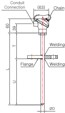
Model No. | SS-5045S (Sheath)
