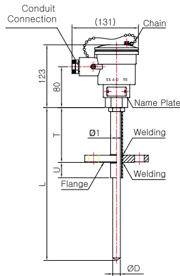
Model No. | SS-5046E-3 (Sheath)
