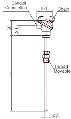
Model No. | SS-5042S-4 (Sheath)
