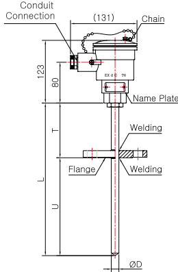
Model No. | SS-5045E (Sheath)
