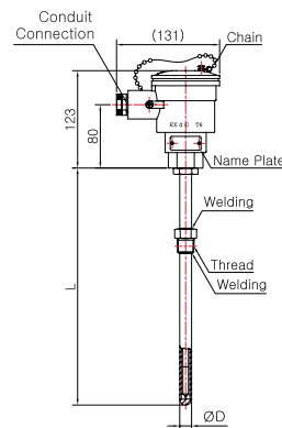
Model No. | SS-5012E-1 (Metal Protection Tube)
