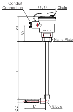
Model No. | SS-5017E ( Metal Protection Tube )
