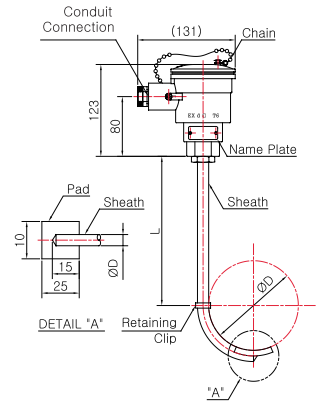
Model No. | SS-5049W-A ( Metal Protection Tube )
