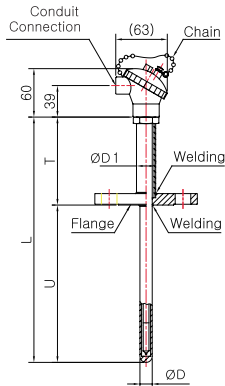
Model No. | SS-5012S-3 ( Metal Protection Tube )
