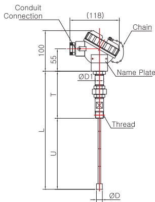
Model No. | SS-5014W-2-1 ( Metal Protection Tube )
