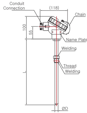
Model No. | SS-5042W-1 (Sheath)
