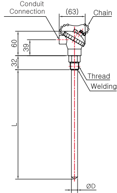
Model No. | SS-5042S (Sheath)
