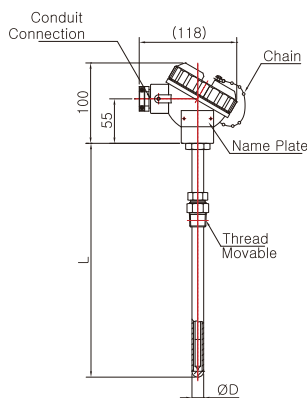
Model No. | SS-5012W-4 ( Metal Protection Tube )
