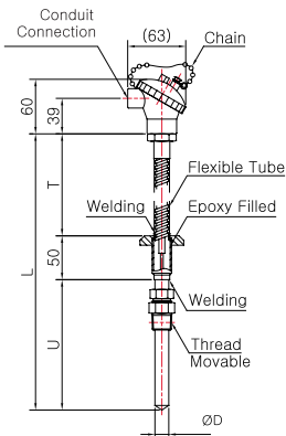
Model No. | SS-5049S-3 (Sheath)
