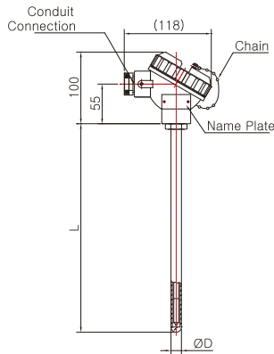
Model No. | SS-5011W-1 ( Ceramic Protection Tube )
