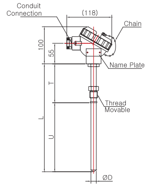
Model No. | SS-5042W-2 (Sheath)
