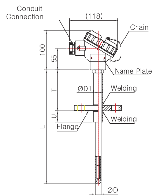
Model No. | SS-5016W-3 ( Metal Protection Tube )
