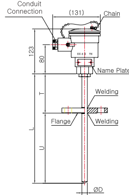
Model No. | SS-5046E-1 (Sheath)
