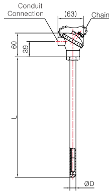
Model No. | SS-5014S-1 ( Metal Protection Tube )
