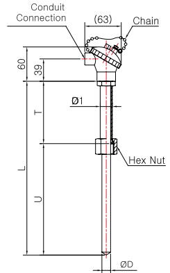
Model No. | SS-5043S-1 (Sheath)
