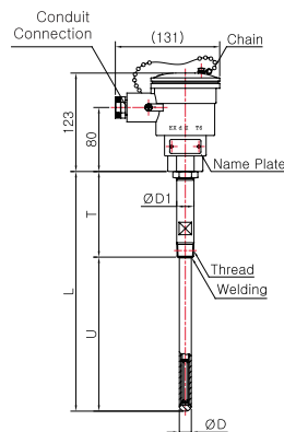
Model No. | SS-5034E-1 ( Metal Protection Tube )
