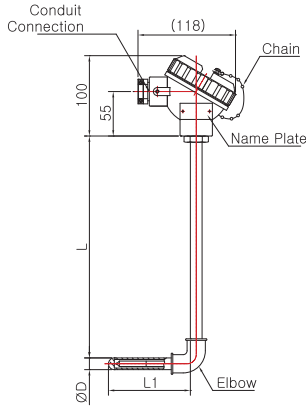
Model No. | SS-5017W ( Metal Protection Tube )
