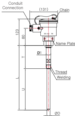
Model No. | SS-5044E-1 (Sheath)
