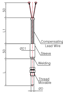
Model No. | SS-5048GDT ( Compensating Lead Wire )
