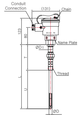
Model No. | SS-5013E-1 ( Metal Protection Tube )
