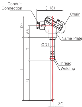
Model No. | SS-5044W-1 (Sheath)
