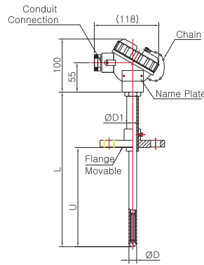
Model No. | SS-5036W-2 ( Metal Protection Tube )
