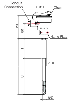
Model No. | SS-5011E-3 (Dual Ceramic Protection Tube)
