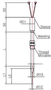
Model No. | SS-5048GD-2 ( Sheath )
