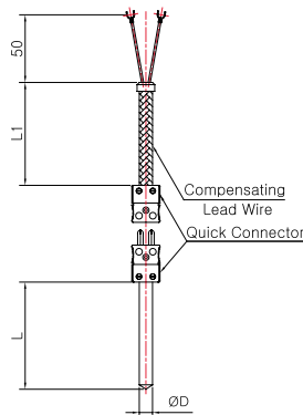
Model No. | SS-5048GG ( Quick Connector )
