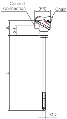
Model No. | SS-5014S ( Ceramic Protection Tube )
