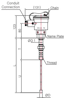
Model No. | SS-5014E-2-1 ( Metal Protection Tube )
