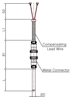
Model No. | SS-5048GH ( Metal Connector )
