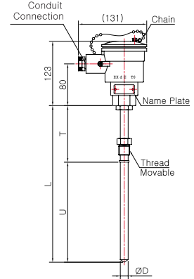
Model No. | SS-5042E-2 (Sheath)
