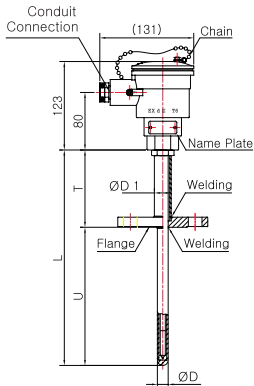
Model No. | SS-5016E ( Metal Protection Tube )
