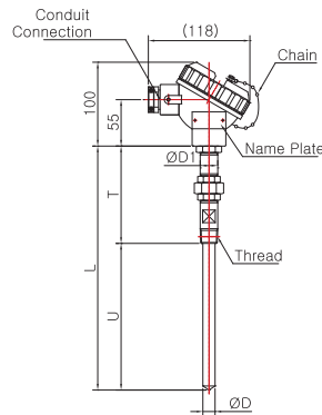
Model No. | SS-5044W-2 (Sheath)
