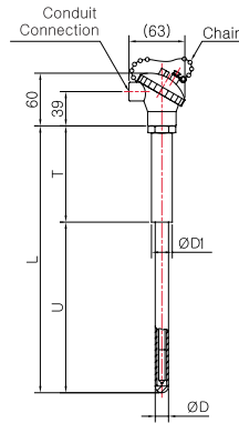
Model No. | SS-5014S-1-1 ( Metal Protection Tube )
