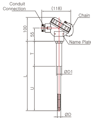
Model No. | SS-5011W-2 ( Ceramic Protection Tube )
