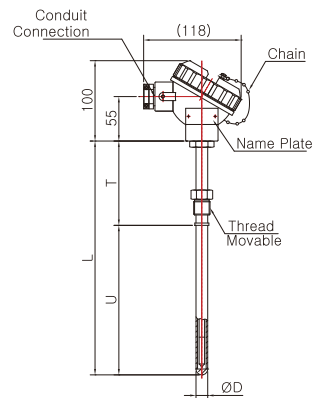
Model No. | SS-5012W-2 ( Metal Protection Tube )
