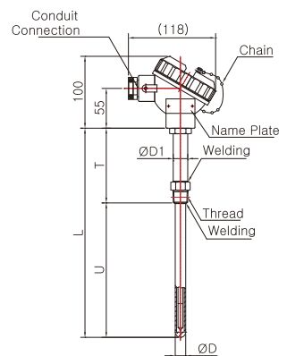
Model No. | SS-5013W ( Ceramic Protection Tube )
