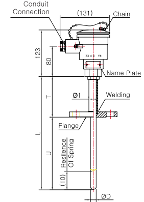
Model No. | SS-5046E-1-1 (Sheath Spring Load)
