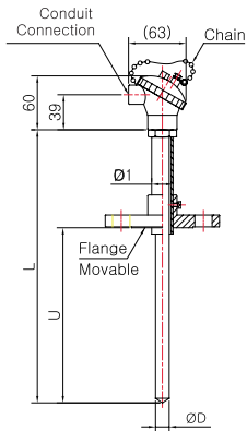
Model No. | SS-5046S-2 (Sheath)
