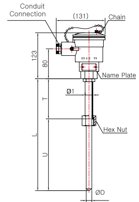
Model No. | SS-5043E-1 (Sheath)
