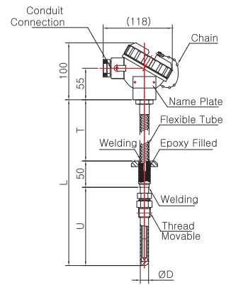
Model No. | SS-5019W-2 ( Metal Protection Tube )
