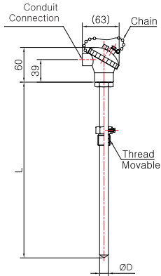
Model No. | SS-5042S-3 (Sheath)
