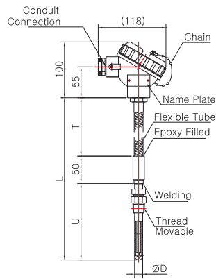
Model No. | SS-5019W-1 ( Metal Protection Tube )
