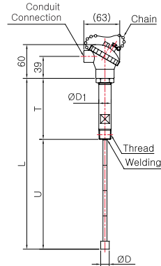
Model No. | SS-5011S-2 ( Ceramic Protection Tube )
