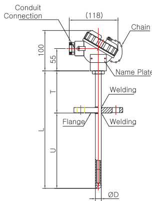
Model No. | SS-5015W ( Metal Protection Tube )
