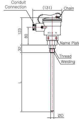
Model No. | SS-5042E-1 (Sheath)
