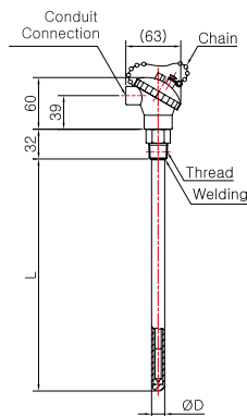
Model No. | SS-5014S-3 ( Metal Protection Tube )
