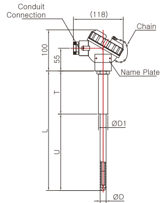
Model No. | SS-5011W-3 ( Dual Ceramic Protection Tube )
