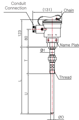
Model No. | SS-5044E-2 (Sheath)
