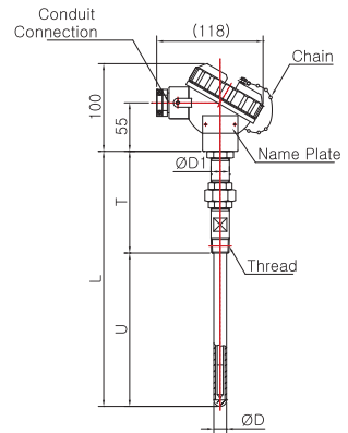
Model No. | SS-5014W-2 ( Metal Protection Tube )
