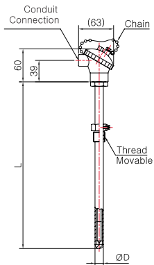
Model No. | SS-5016S ( Metal Protection Tube )
