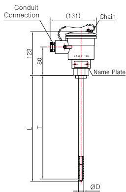
Model No. | SS-5011E-4 (Metal Protection Tube)
