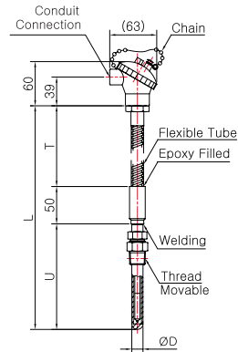
Model No. | SS-5019S-1 ( Metal Protection Tube )
