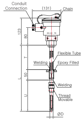
Model No. | SS-5019E-2 ( Metal Protection Tube )
