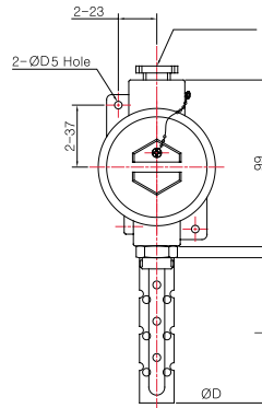
Model No. | SS-5048GC ( Compensating Lead Wire )
