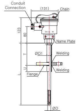
Model No. | SS-5016E-3 ( Metal Protection Tube )
