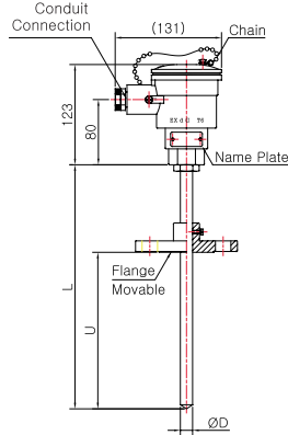
Model No. | SS-5045E-1 (Sheath)
