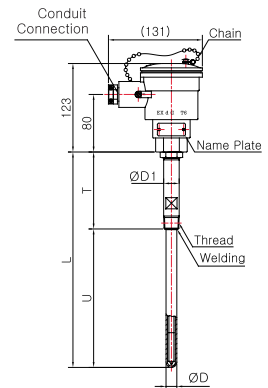
Model No. | SS-5013E-1 (Ceramic Protection Tube)
