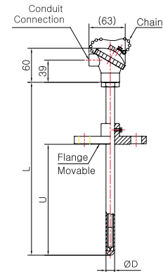
Model No. | SS-5012S-2 ( Metal Protection Tube )
