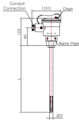
Model No. | SS-5011E-1 (Ceramic Protection Tube)
