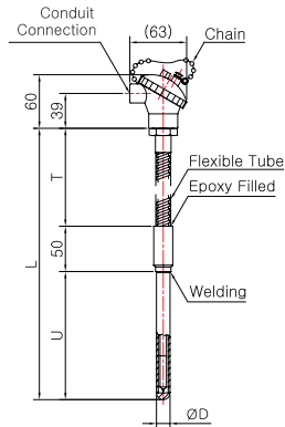
Model No. | SS-5019S ( Metal Protection Tube )
