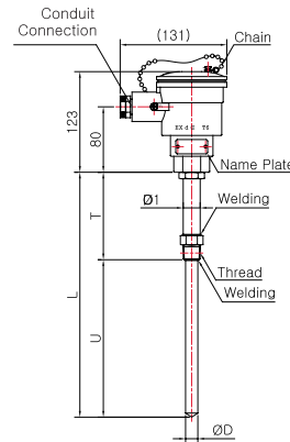
Model No. | SS-5043E (Sheath)
