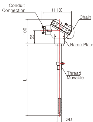
Model No. | SS-5012W-3 ( Metal Protection Tube )
