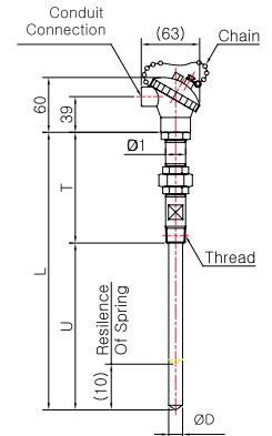
Model No. | SS-5044S-2-1 (Sheath Spring Load)
