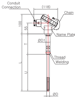
Model No. | SS-5014W ( Ceramic Protection Tube )
