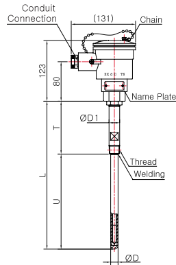
Model No. | SS-5014E-1 ( Metal Protection Tube )
