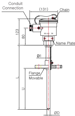
Model No. | SS-5046E-2 (Sheath)
