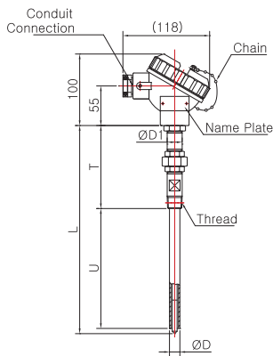
Model No. | SS-5014W-3 ( Metal Protection Tube )
