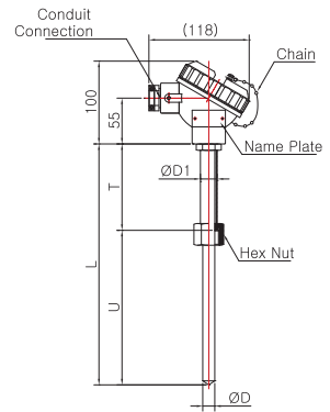
Model No. | SS-5043W-1 (Sheath)
