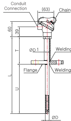
Model No. | SS-5012S-4 ( Metal Protection Tube )
