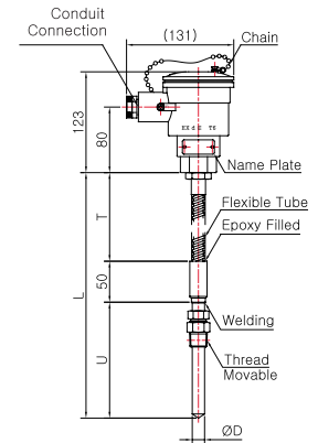
Model No. | SS-5049E-1 (Sheath)
