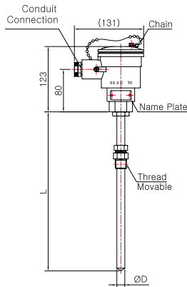
Model No. | SS-5042E-4 (Sheath)
