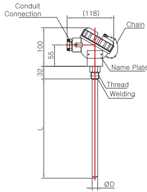
Model No. | SS-5042W (Sheath)
