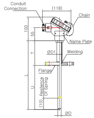
Model No. | SS-5046W-1-1 (Sheath Spring Load)
