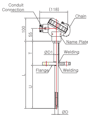
Model No. | SS-5016W ( Metal Protection Tube )
