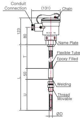
Model No. | SS-5019E-1 ( Metal Protection Tube )
