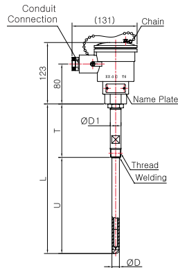
Model No. | SS-5014E-3 ( Metal Protection Tube )
