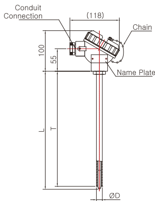
Model No. | SS-5011W-4 ( Metal Protection Tube )
