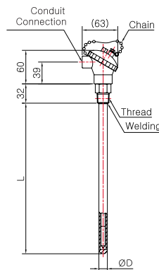
Model No. | SS-5015S ( Metal Protection Tube )
