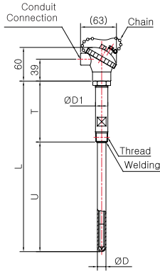
Model No. | SS-5011S ( Ceramic Protection Tube )
