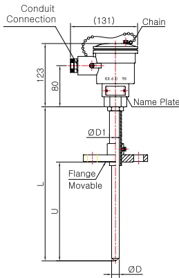
Model No. | SS-5026E-2 (Sheath)
