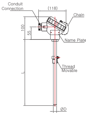
Model No. | SS-5042W-3 (Sheath)
