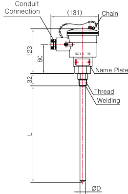
Model No. | SS-5042E (Sheath)
