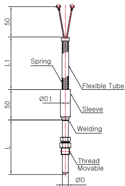
Model No. | SS-5048GET ( Flexible Tube )
