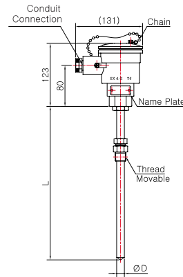
Model No. | SS-5023E (Sheath)
