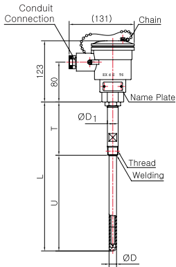
Model No. | SS-5014E ( Ceramic Protection Tube )
