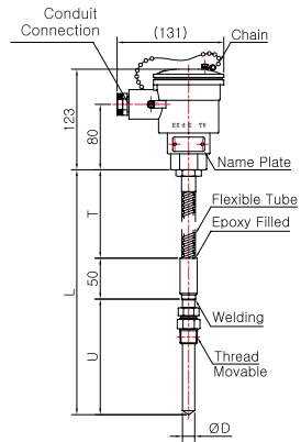
Model No. | SS-5029E-1 (Sheath)
