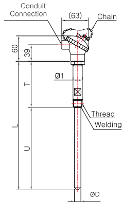
Model No. | SS-5044S-1-1 (Sheath Spring Load)
