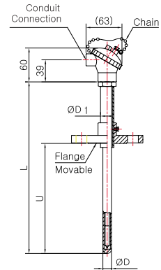
Model No. | SS-5013S ( Metal Protection Tube )
