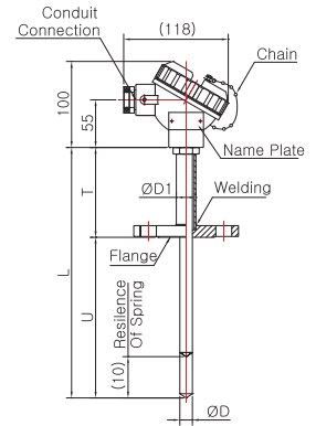
Model No. | SS-5026W-1-1 (Sheath Spring Load)
