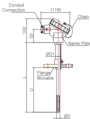
Model No. | SS-5016W-2 ( Metal Protection Tube )
