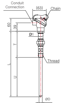
Model No. | SS-5044S-2 (Sheath)
