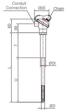
Model No. | SS-5014S-2 ( Metal Protection Tube )
