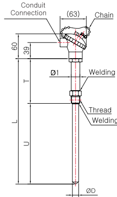
Model No. | SS-5043S (Sheath)
