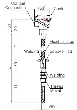
Model No. | SS-5019S-2 ( Metal Protection Tube )
