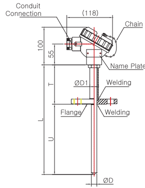
Model No. | SS-5046W-1 (Sheath)
