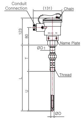
Model No. | SS-5014E-2 ( Metal Protection Tube )
