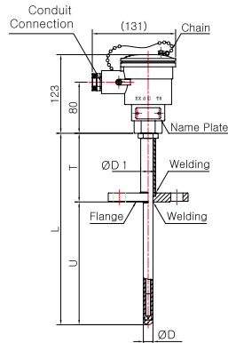
Model No. | SS-5016E-1 ( Ceramic Protection Tube )
