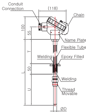
Model No. | SS-5049W-3 (Sheath)
