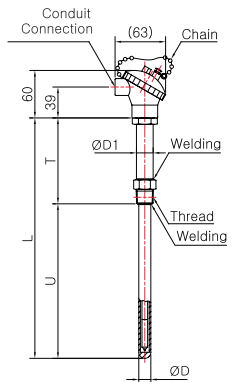
Model No. | SS-5016S-3 ( Metal Protection Tube )
