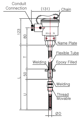
Model No. | SS-5039E-2 ( Metal Protection Tube )
