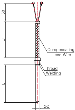
Model No. | SS-5048GD-1 ( Compensating Lead Wire )
