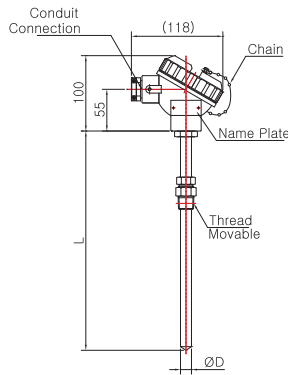
Model No. | SS-5042W-4 (Sheath)
