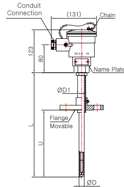
Model No. | SS-5016E-1 ( Metal Protection Tube )
